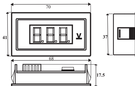
85SDM DIMENSION
