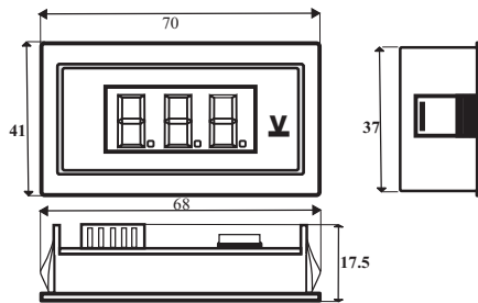
85SDM DIMENSION
